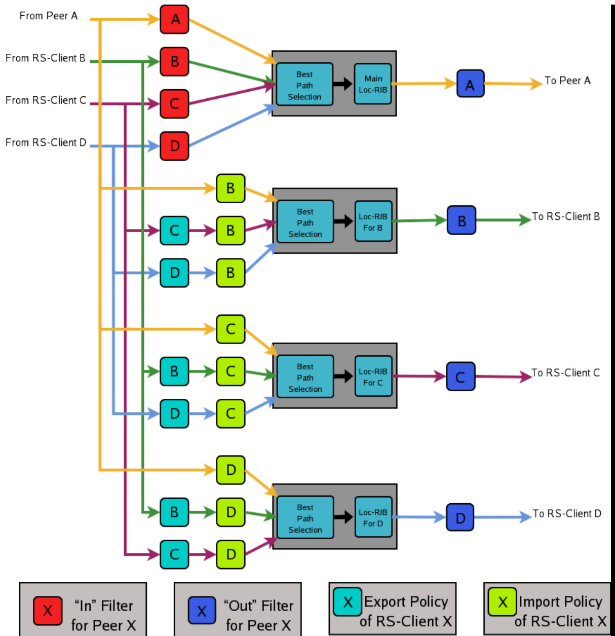
Figure 11.4: Announcement processing model implemented by the Route Server
