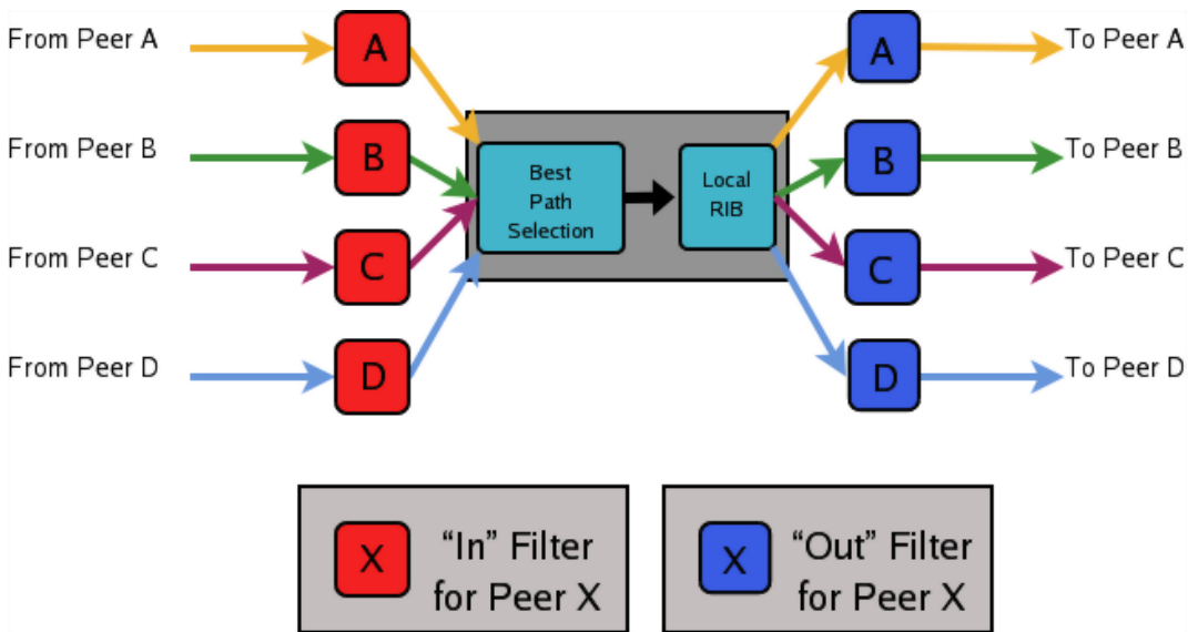
Figure 11.1: Announcement processing inside a “normal” BGP speaker
