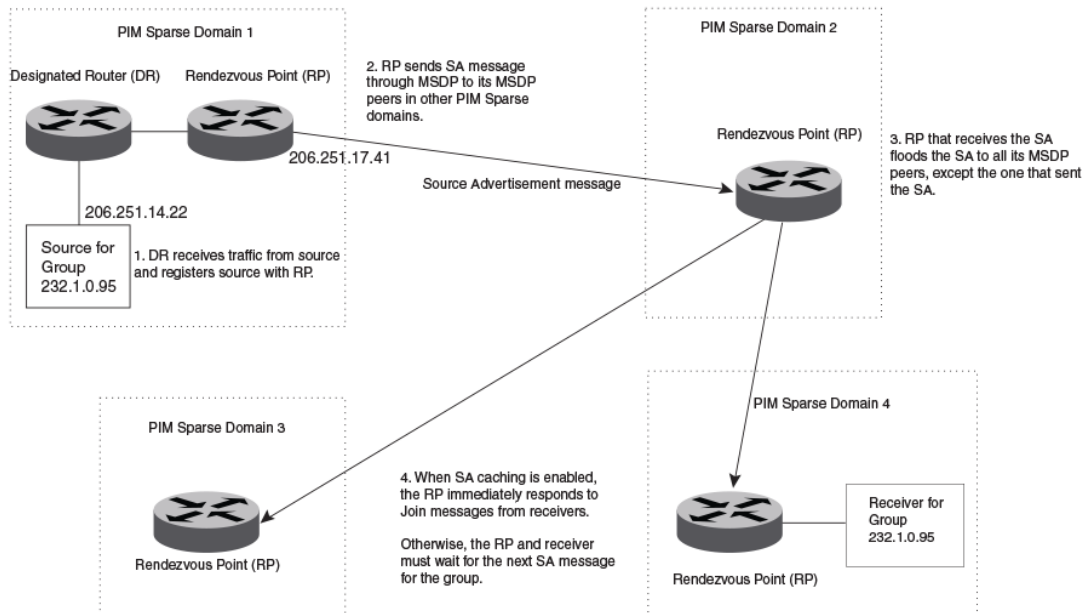
FIGURE 7 PIM Sparse domains joined by MSDP devices
