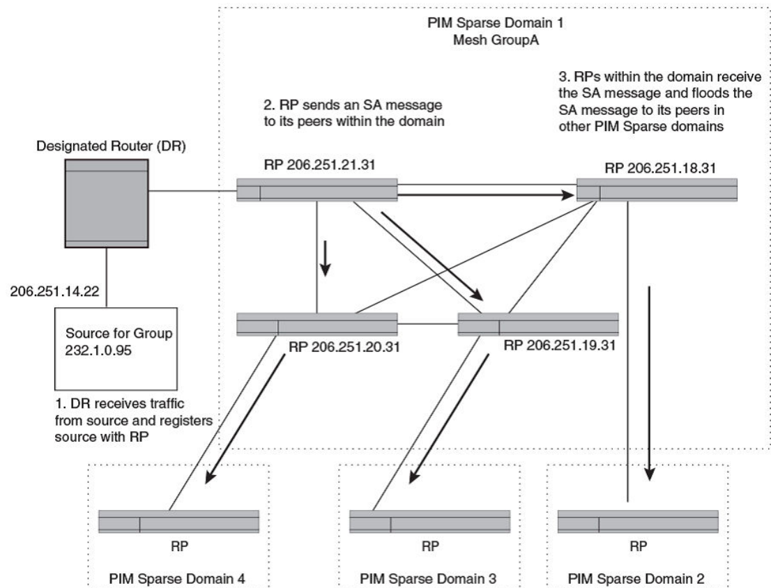
FIGURE 8 Example of MSDP mesh group
