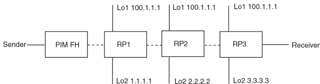
FIGURE 10 Example of a PIM Anycast RP network
