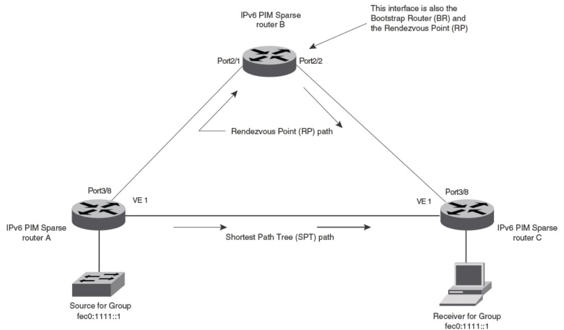
FIGURE 11 Example IPv6 PIM Sparse domain
