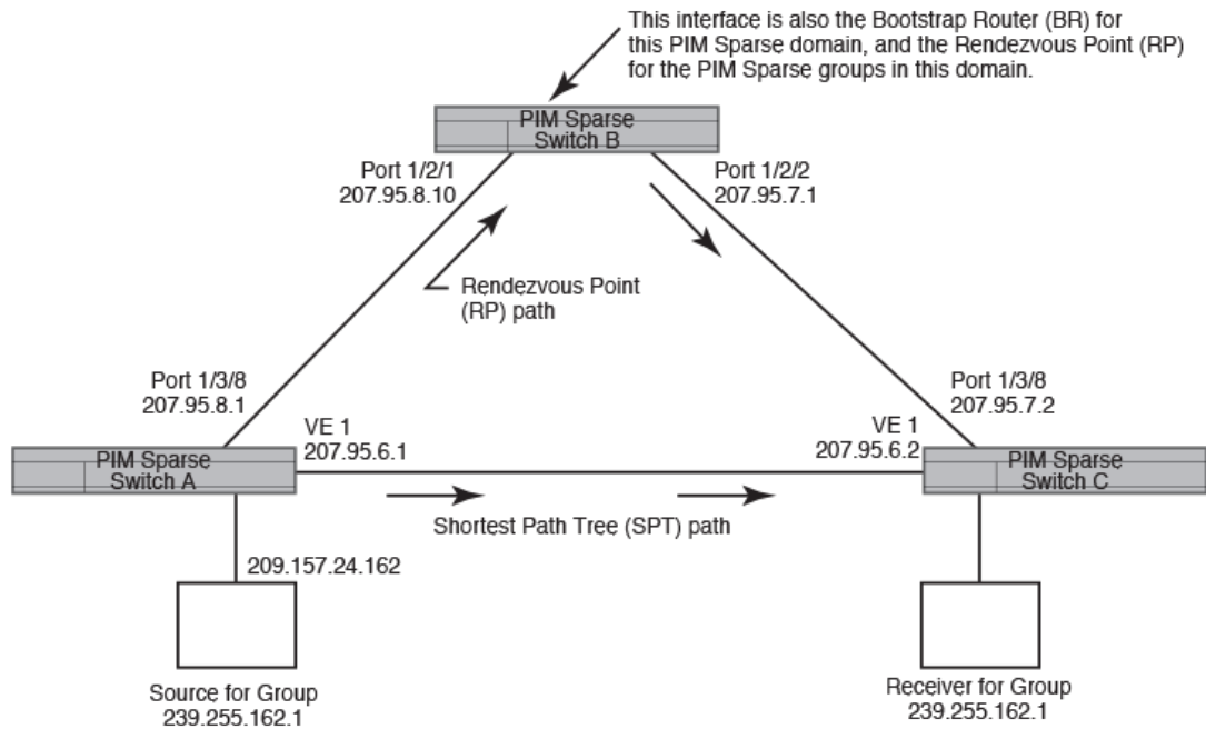
FIGURE 5 Example PIM Sparse domain
