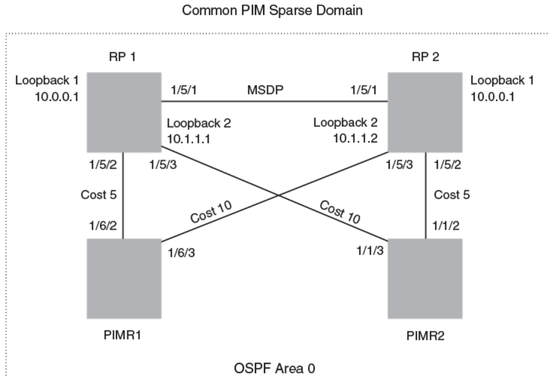
FIGURE 9 Example of a MSDP Anycast RP network
